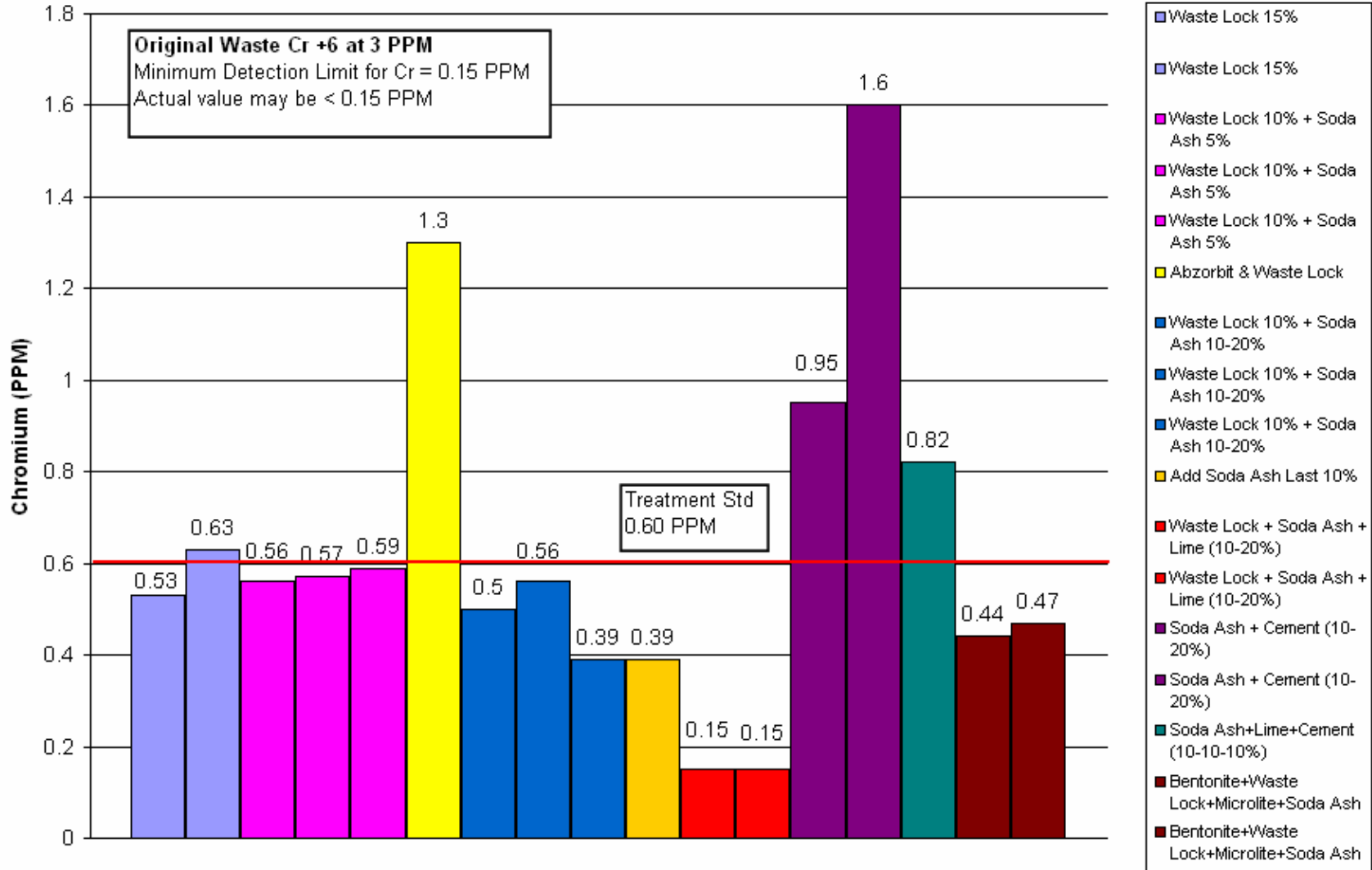
Treatability Results for Chromium (+6) (TCLP)
